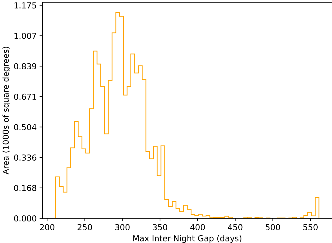
too_elab_r16_d2_gz_v3.4_10yrs WFD r band: Max Inter-Night Gap
