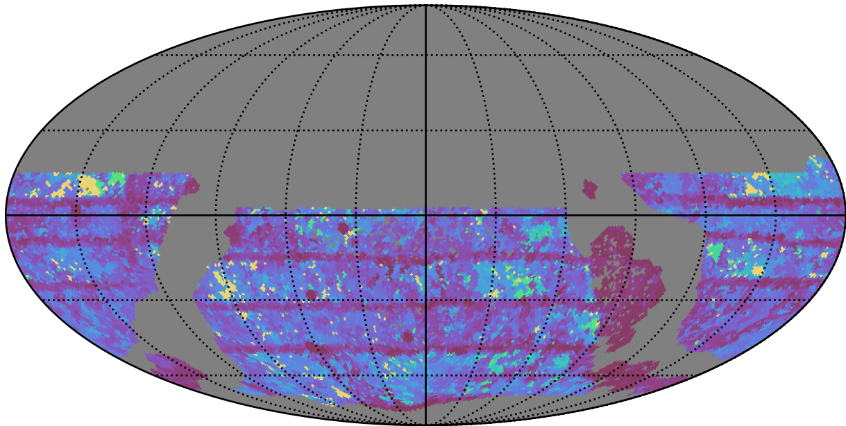
too_elab_r16_d2_gz_v3.4_10yrs WFD i band: Max Inter-Night Gap
