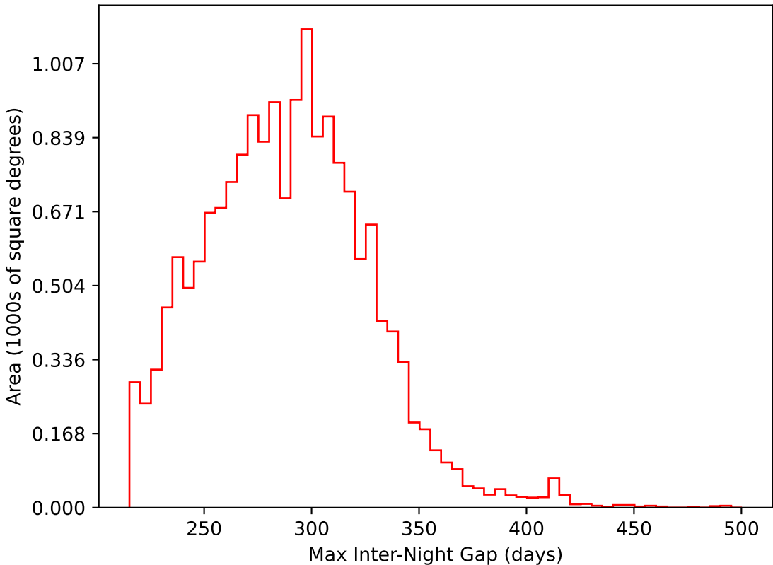
too_elab_r16_d2_gz_v3.4_10yrs WFD i band: Max Inter-Night Gap
