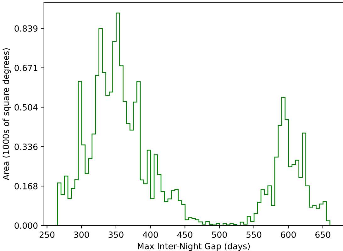
too_elab_r16_d2_gz_v3.4_10yrs WFD g band: Max Inter-Night Gap
