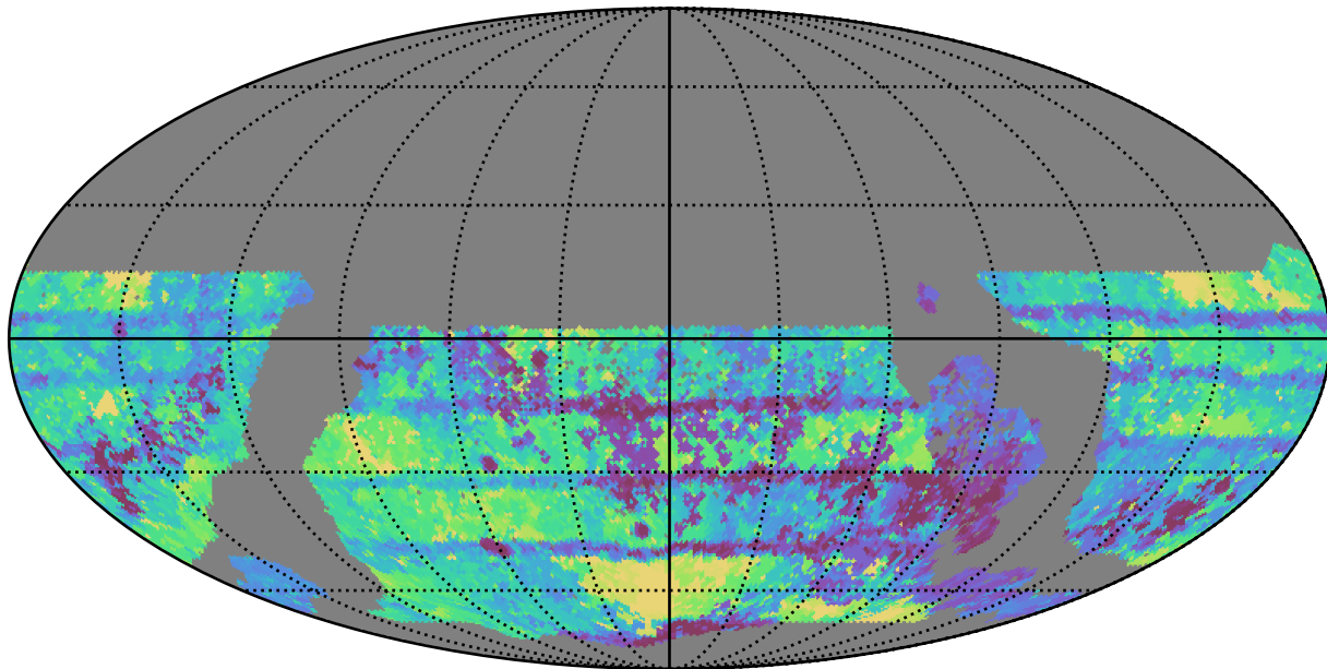
too_elab_r16_d2_gz_v3.4_10yrs WFD all bands: Max Inter-Night Gap
