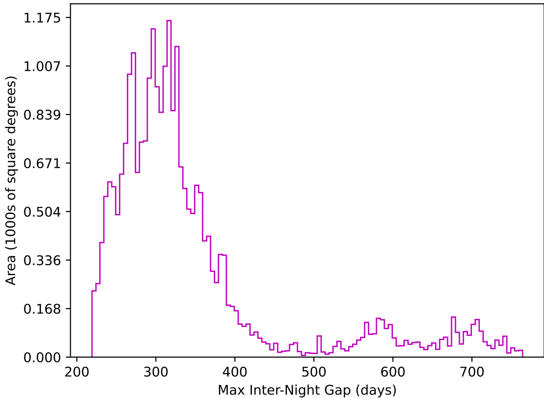
too_elab_r16_d2_gz_v3.4_10yrs All sky z band: Max Inter-Night Gap
