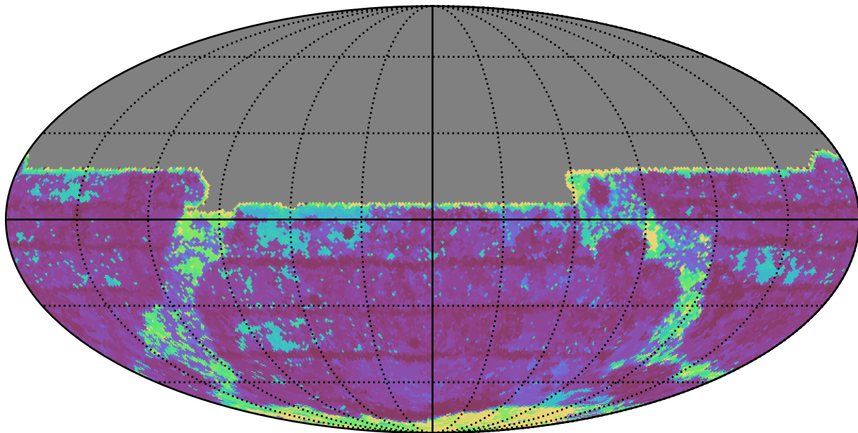
too_elab_r16_d2_gz_v3.4_10yrs All sky y band: Max Inter-Night Gap
