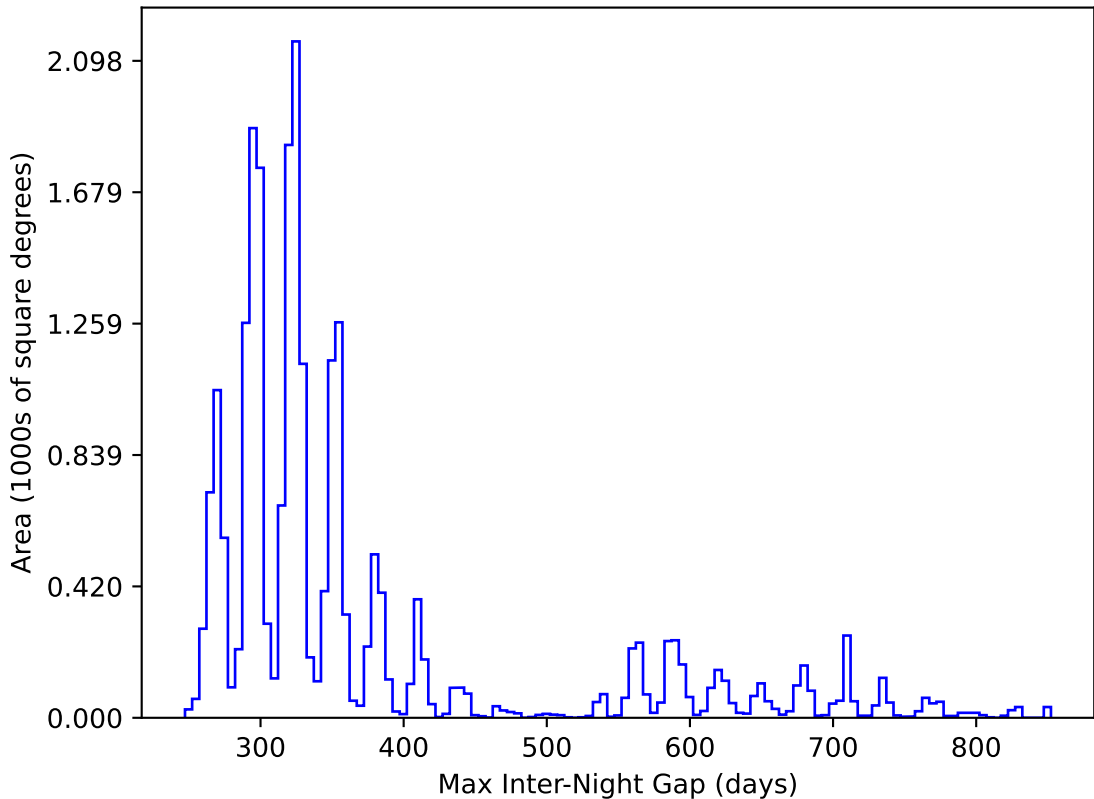
too_elab_r16_d2_gz_v3.4_10yrs All sky y band: Max Inter-Night Gap
