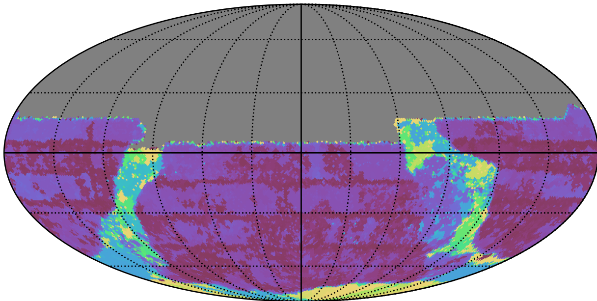
too_elab_r16_d2_gz_v3.4_10yrs All sky u band: Max Inter-Night Gap
