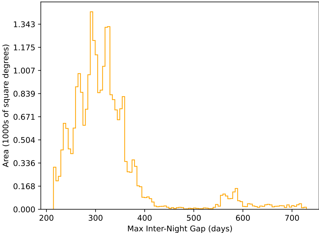
too_elab_r16_d2_gz_v3.4_10yrs All sky r band: Max Inter-Night Gap
