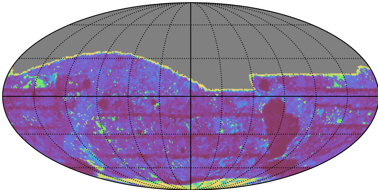
too_elab_r16_d2_gz_v3.4_10yrs All sky i band: Max Inter-Night Gap
