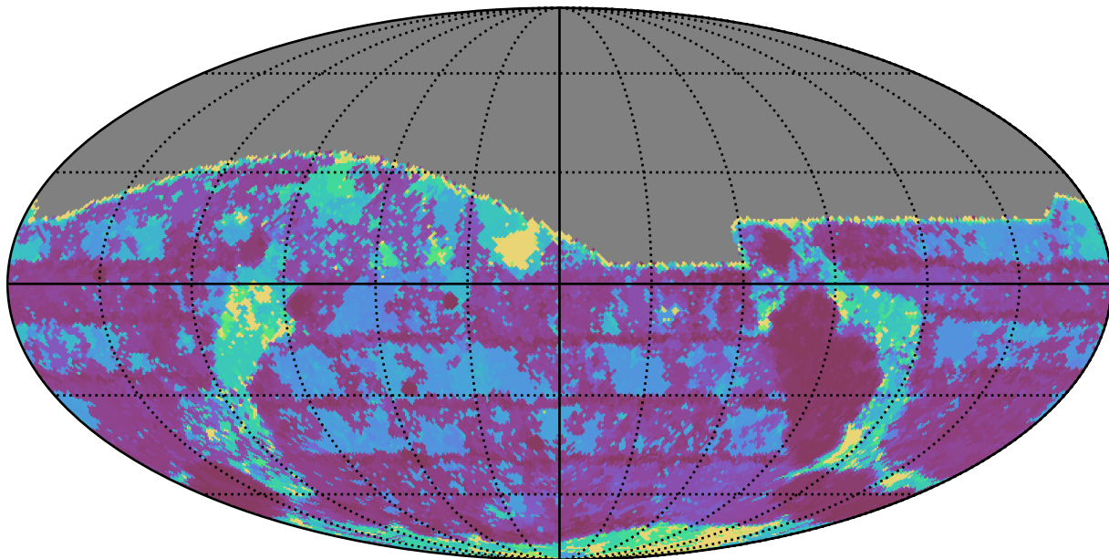
too_elab_r16_d2_gz_v3.4_10yrs All sky g band: Max Inter-Night Gap
