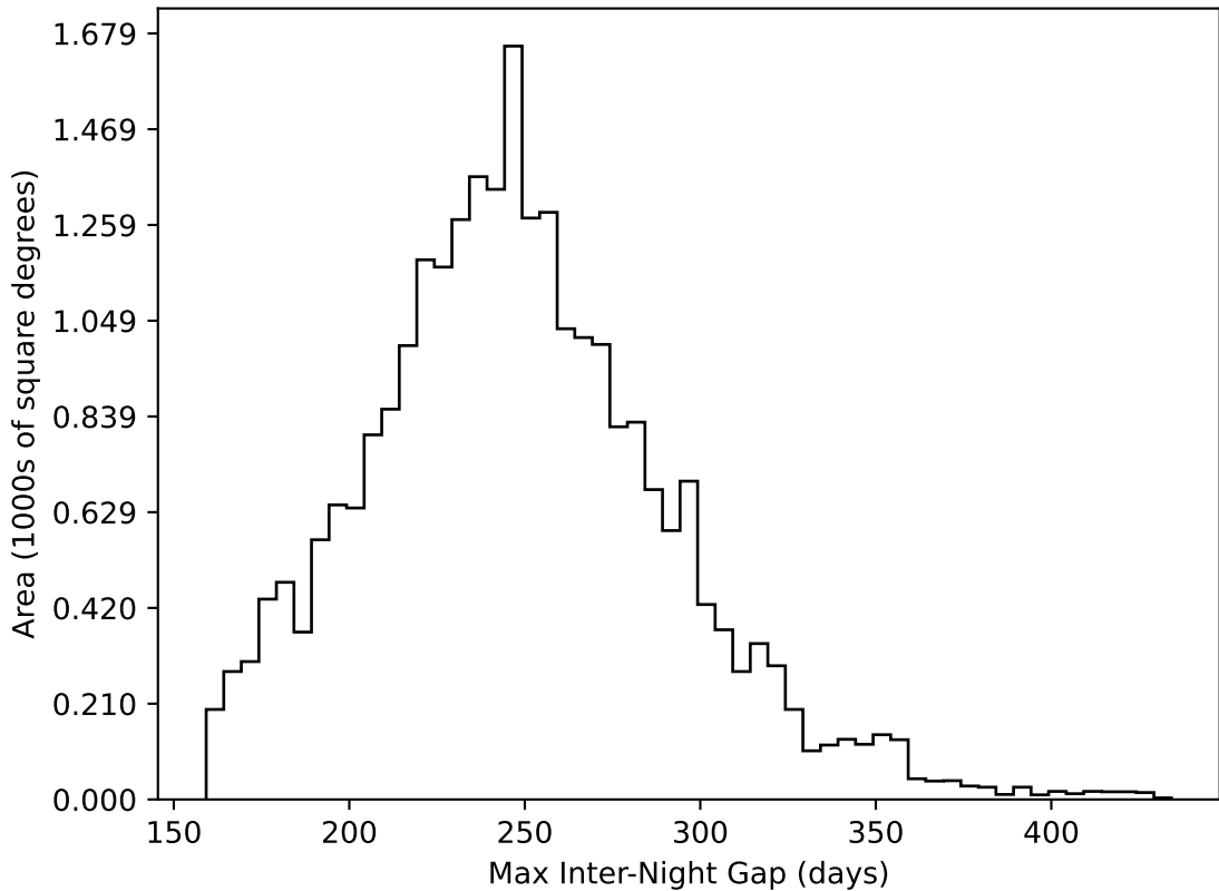
too_elab_r16_d2_gz_v3.4_10yrs All sky all bands: Max Inter-Night Gap
