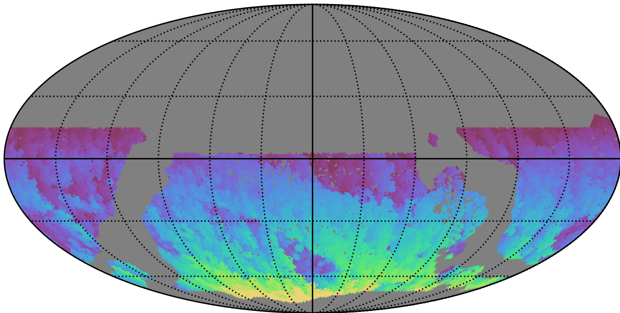
too_elab_r16_d2_gz_v3.4_10yrs WFD z band: Max HA
