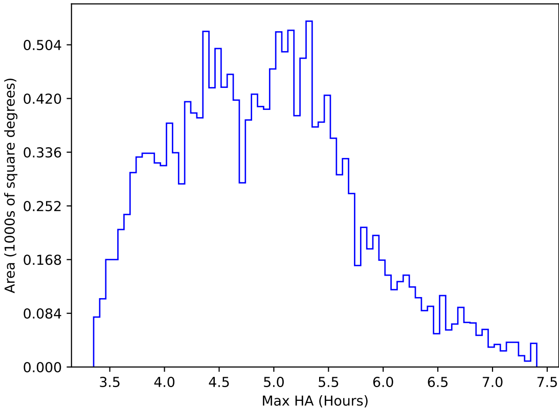
too_elab_r16_d2_gz_v3.4_10yrs WFD z band: Max HA
