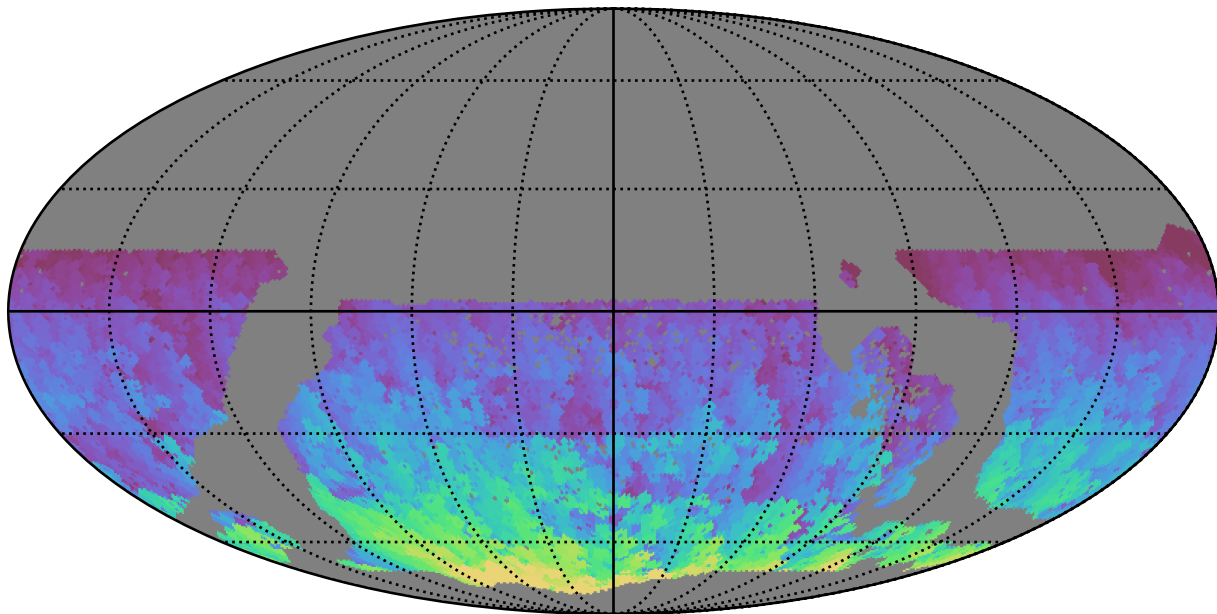
too_elab_r16_d2_gz_v3.4_10yrs WFD y band: Max HA
