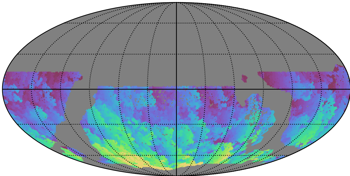
too_elab_r16_d2_gz_v3.4_10yrs WFD u band: Max HA
