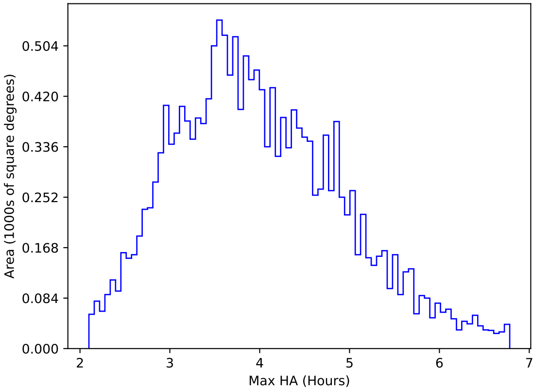
too_elab_r16_d2_gz_v3.4_10yrs WFD u band: Max HA
