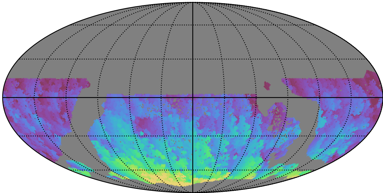
too_elab_r16_d2_gz_v3.4_10yrs WFD r band: Max HA
