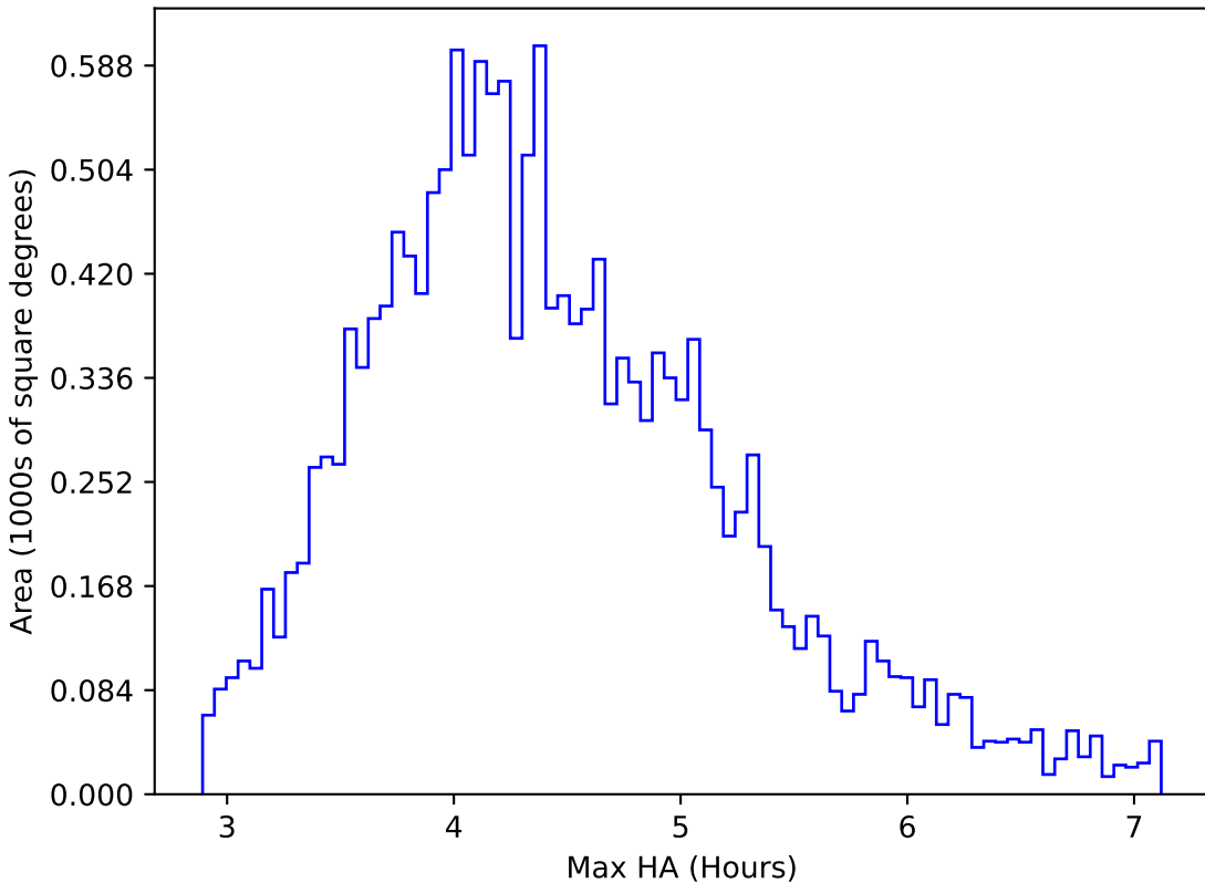
too_elab_r16_d2_gz_v3.4_10yrs WFD r band: Max HA
