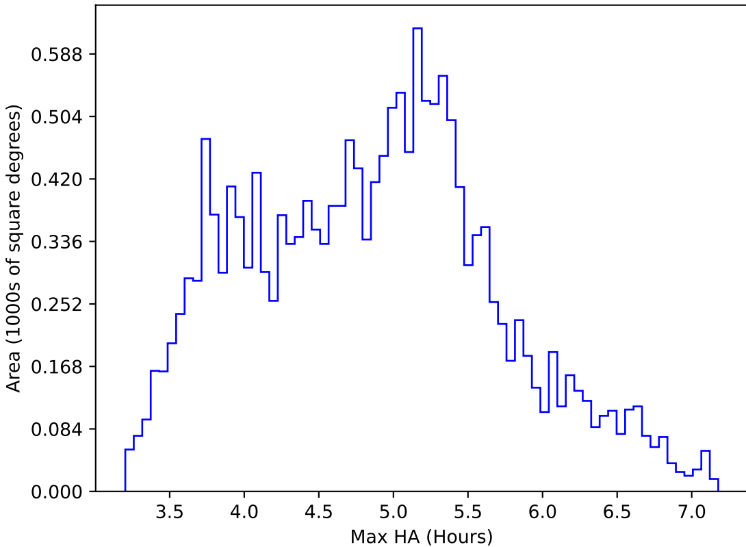
too_elab_r16_d2_gz_v3.4_10yrs WFD i band: Max HA
