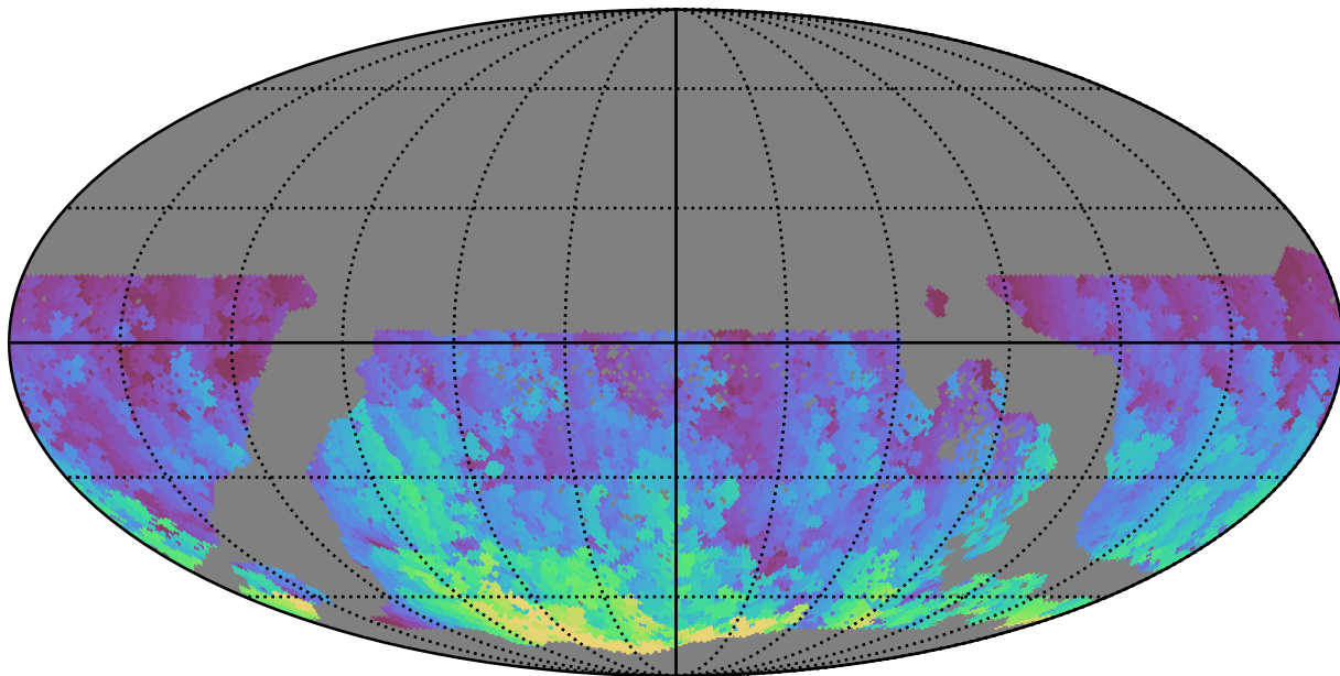
too_elab_r16_d2_gz_v3.4_10yrs WFD g band: Max HA
