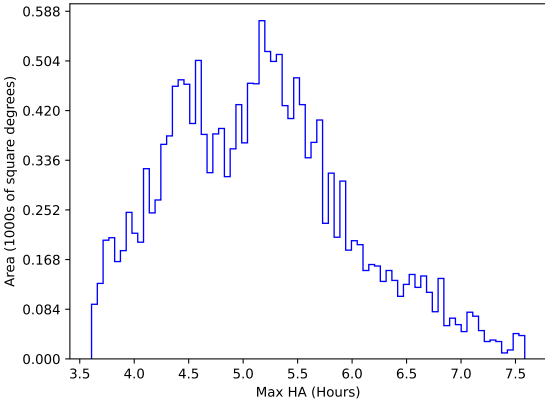
too_elab_r16_d2_gz_v3.4_10yrs WFD all bands: Max HA
