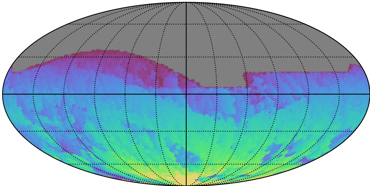
too_elab_r16_d2_gz_v3.4_10yrs All sky z band: Max HA
