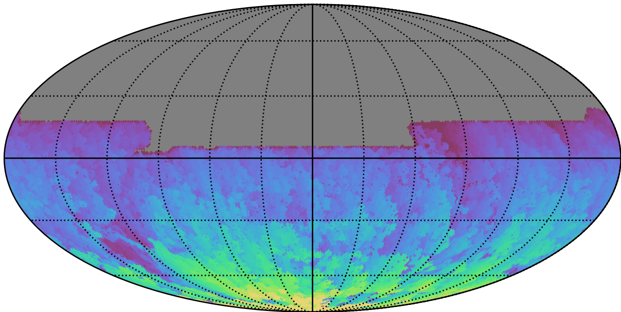
too_elab_r16_d2_gz_v3.4_10yrs All sky y band: Max HA
