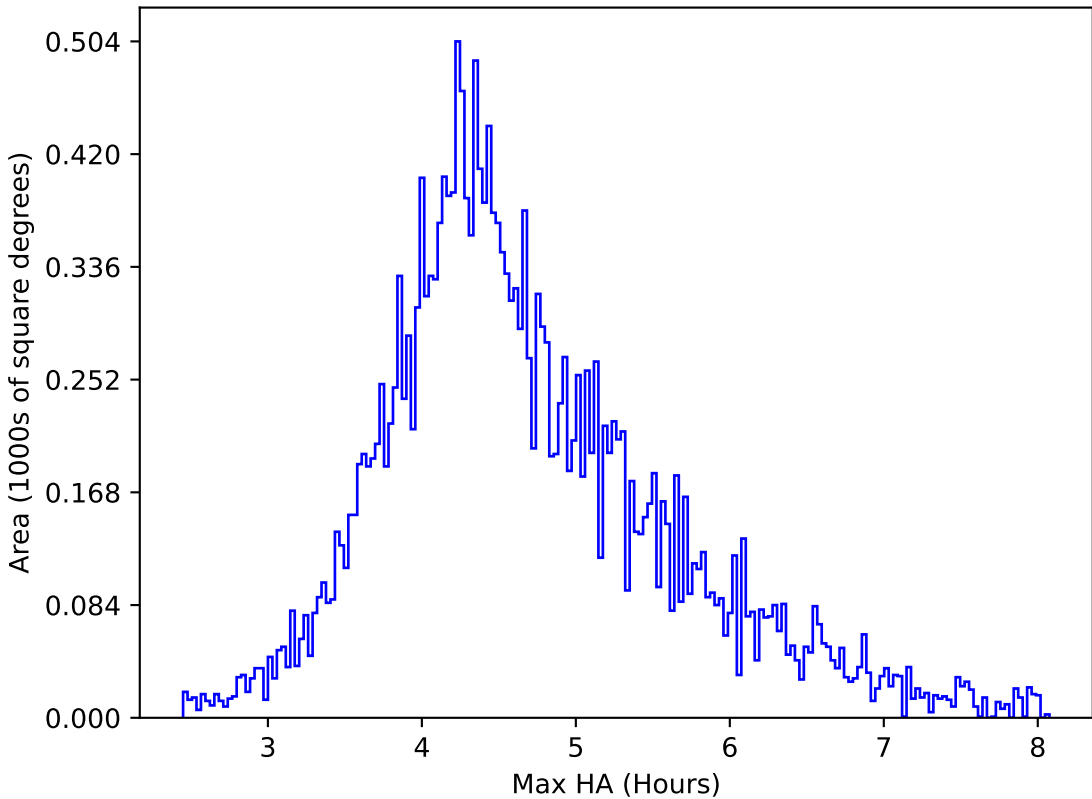
too_elab_r16_d2_gz_v3.4_10yrs All sky y band: Max HA
