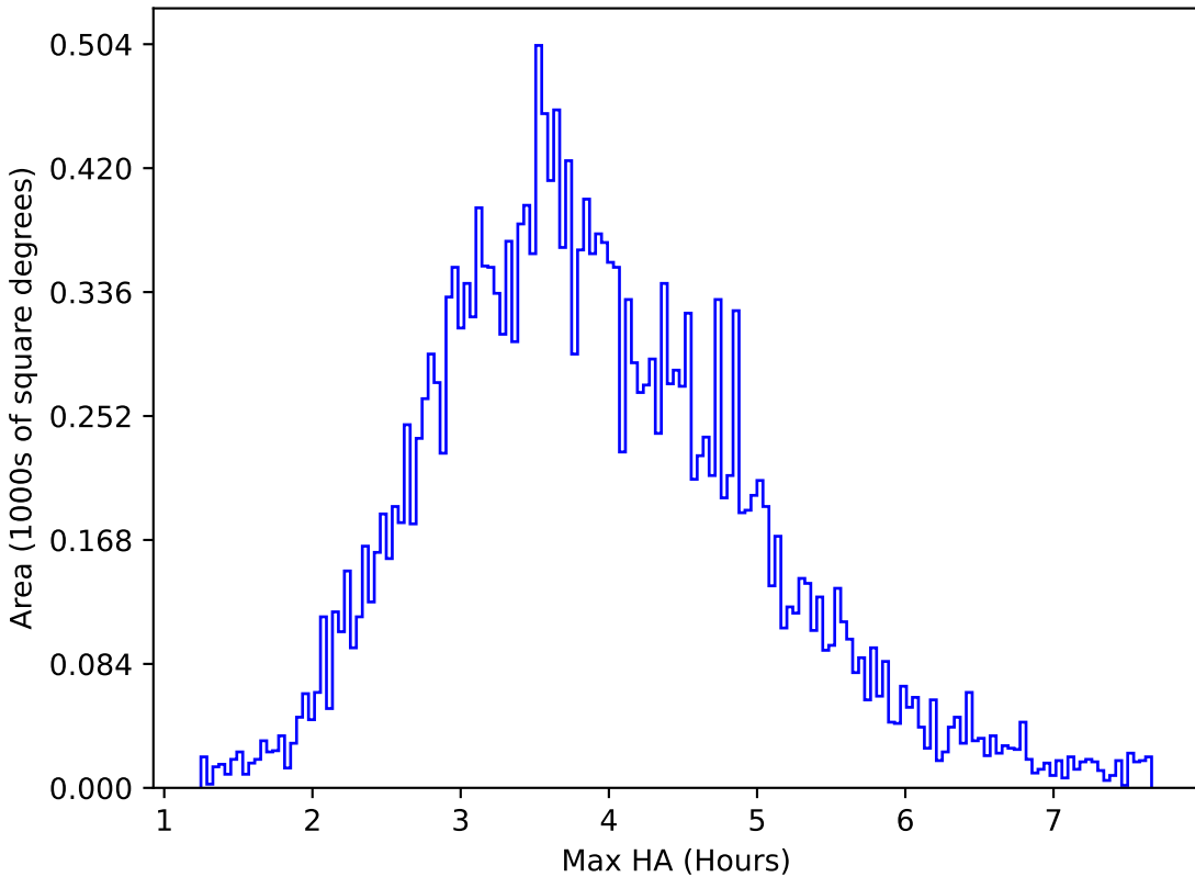
too_elab_r16_d2_gz_v3.4_10yrs All sky u band: Max HA
