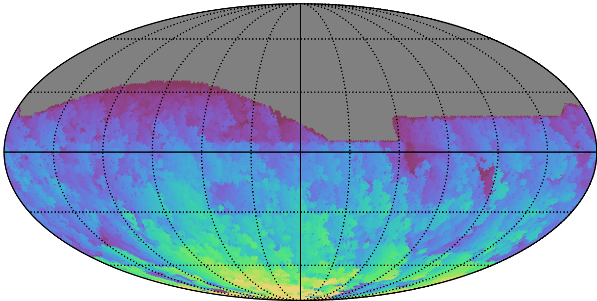
too_elab_r16_d2_gz_v3.4_10yrs All sky r band: Max HA
