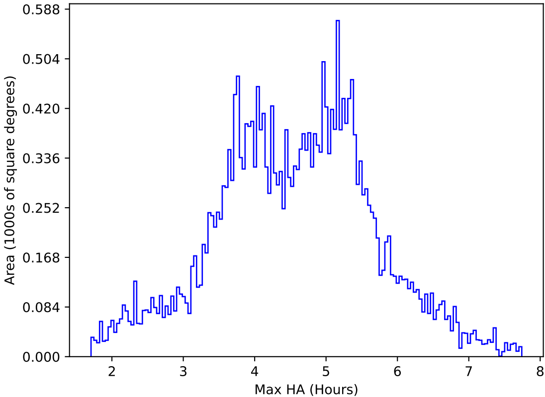
too_elab_r16_d2_gz_v3.4_10yrs All sky i band: Max HA
