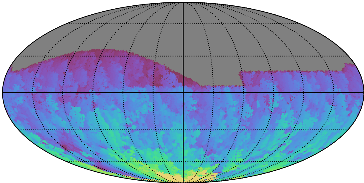
too_elab_r16_d2_gz_v3.4_10yrs All sky g band: Max HA
