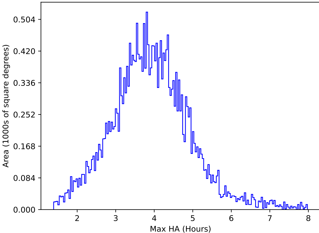
too_elab_r16_d2_gz_v3.4_10yrs All sky g band: Max HA
