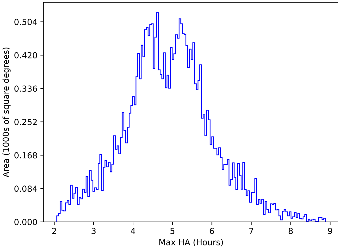
too_elab_r16_d2_gz_v3.4_10yrs All sky all bands: Max HA
