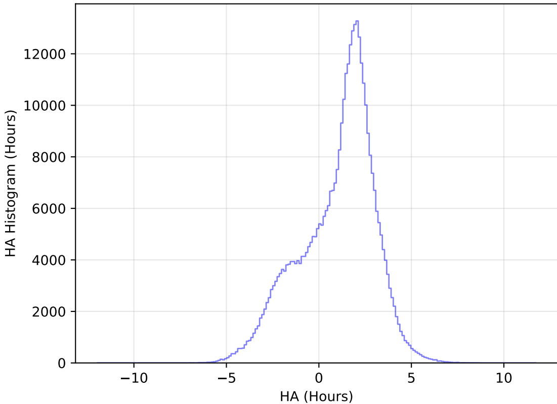
too_elab_r16_d2_gz_v3.4_10yrs WFD y band: HA Histogram
