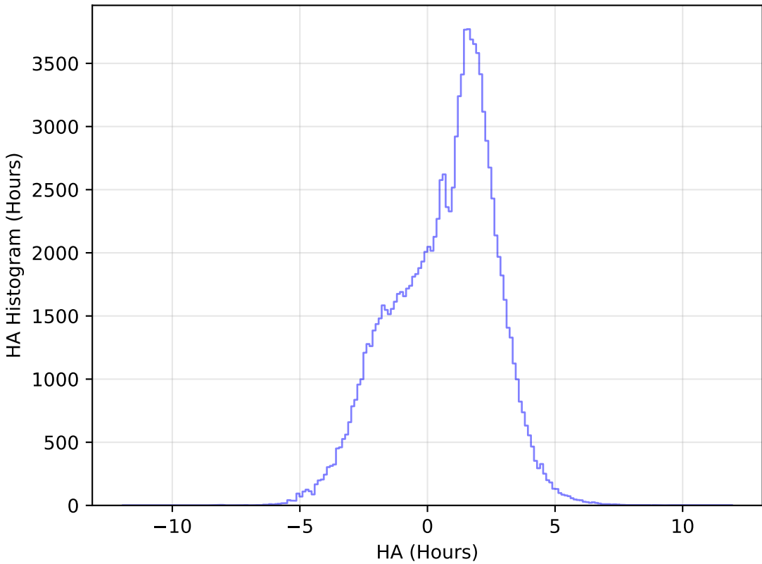
too_elab_r16_d2_gz_v3.4_10yrs WFD u band: HA Histogram
