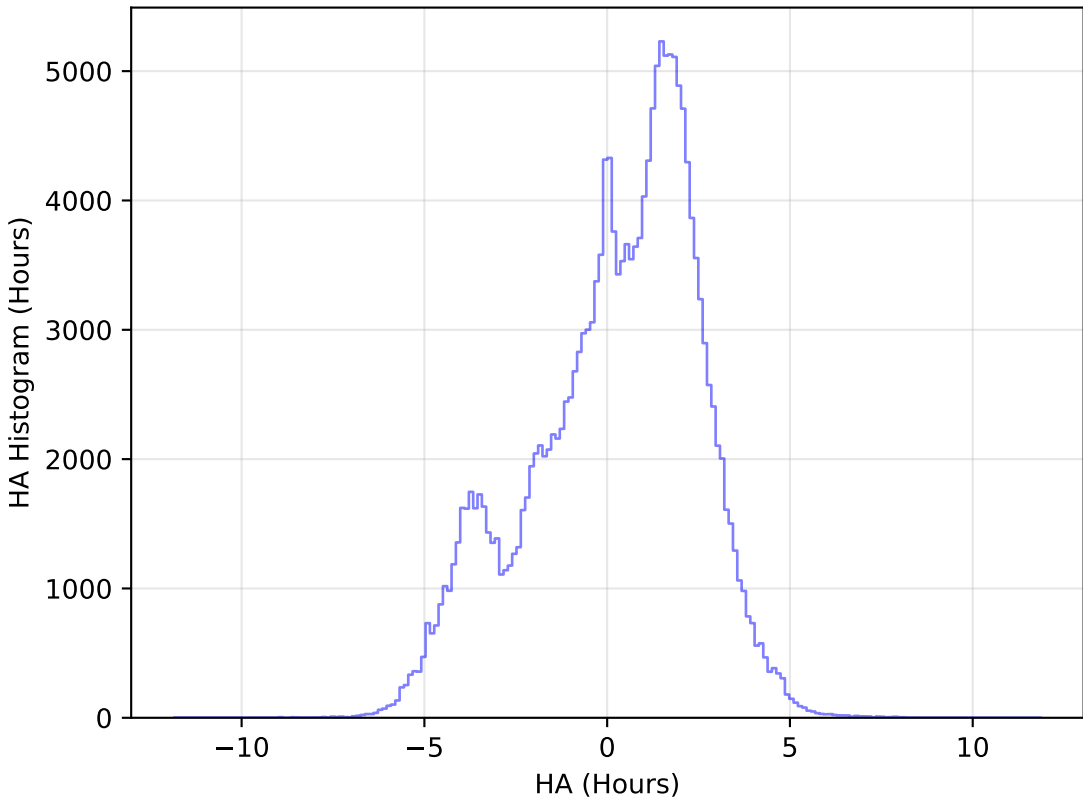
too_elab_r16_d2_gz_v3.4_10yrs WFD g band: HA Histogram
