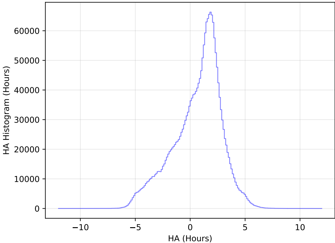
too_elab_r16_d2_gz_v3.4_10yrs WFD all bands: HA Histogram
