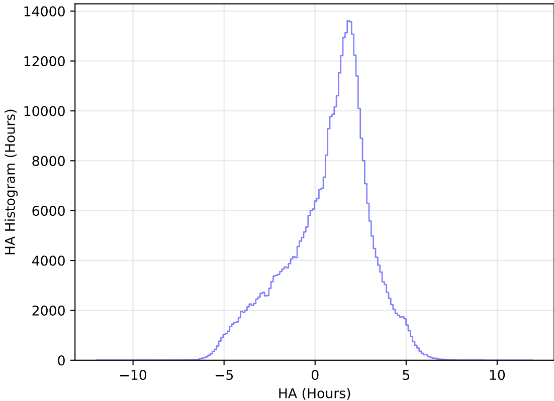
too_elab_r16_d2_gz_v3.4_10yrs All sky z band: HA Histogram
