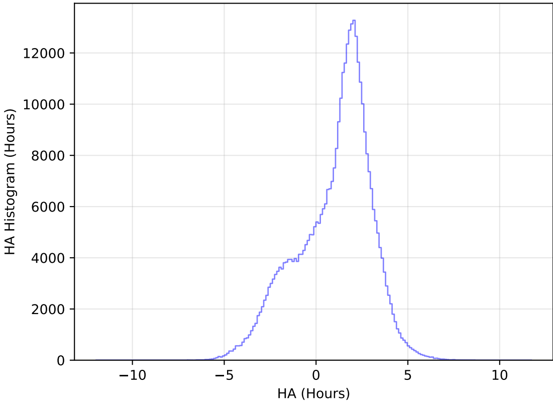
too_elab_r16_d2_gz_v3.4_10yrs All sky y band: HA Histogram
