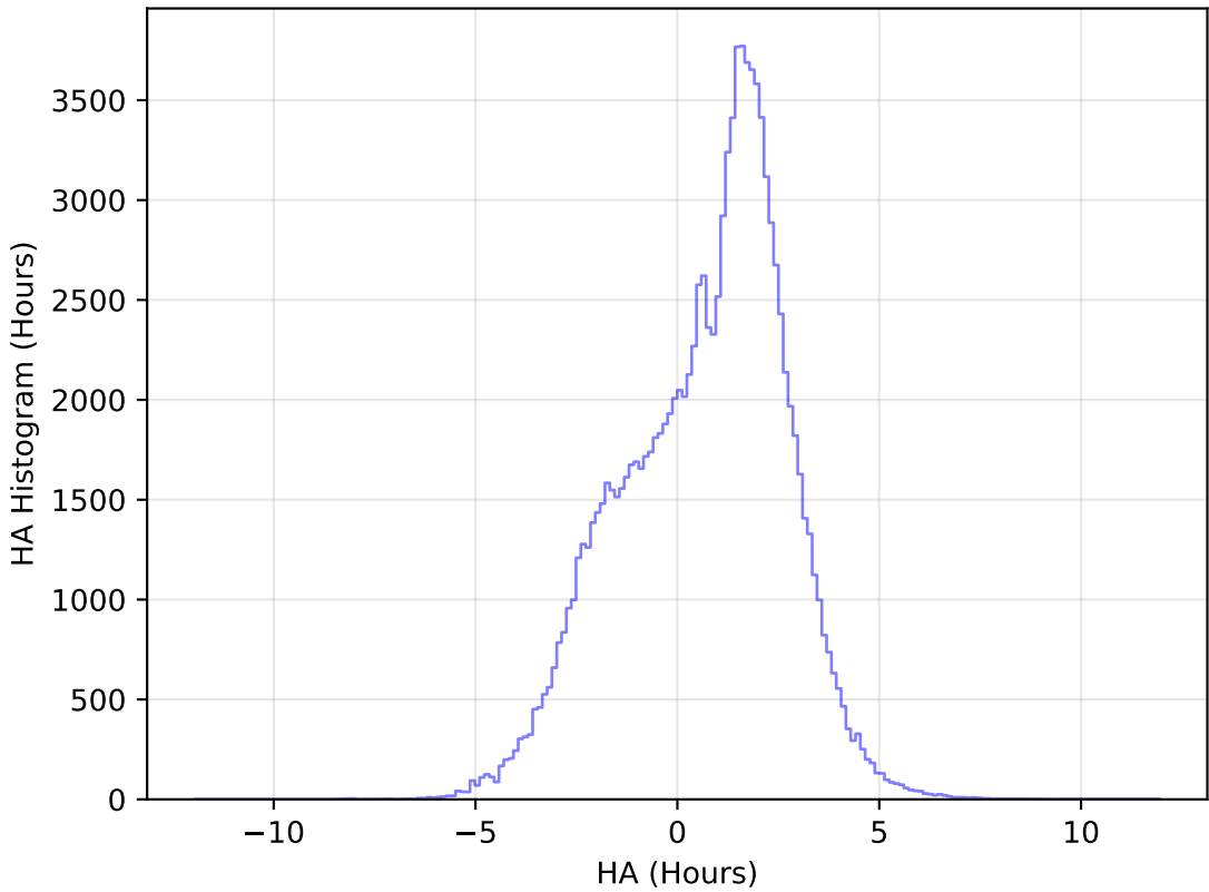
too_elab_r16_d2_gz_v3.4_10yrs All sky u band: HA Histogram
