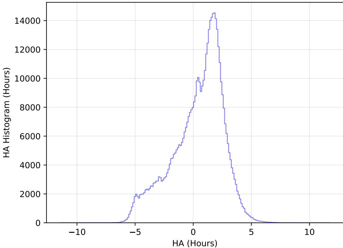
too_elab_r16_d2_gz_v3.4_10yrs All sky r band: HA Histogram
