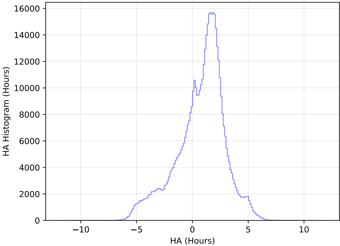
too_elab_r16_d2_gz_v3.4_10yrs All sky i band: HA Histogram
