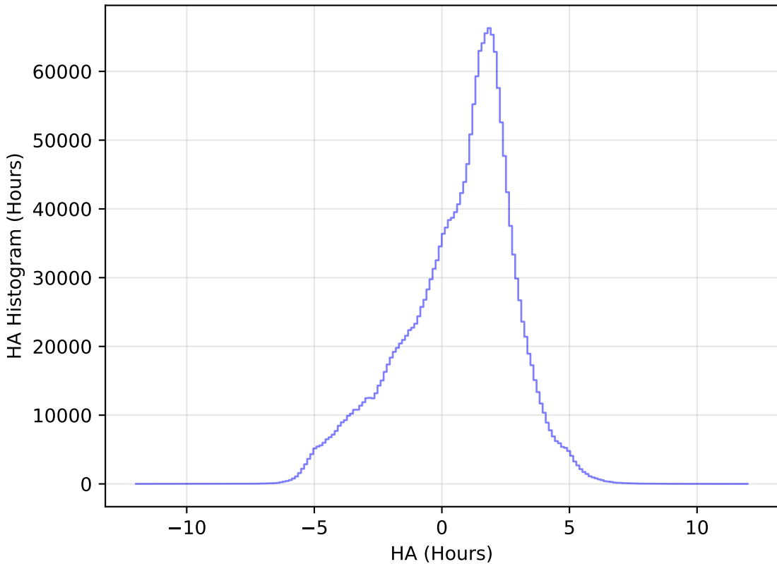
too_elab_r16_d2_gz_v3.4_10yrs All sky all bands: HA Histogram
