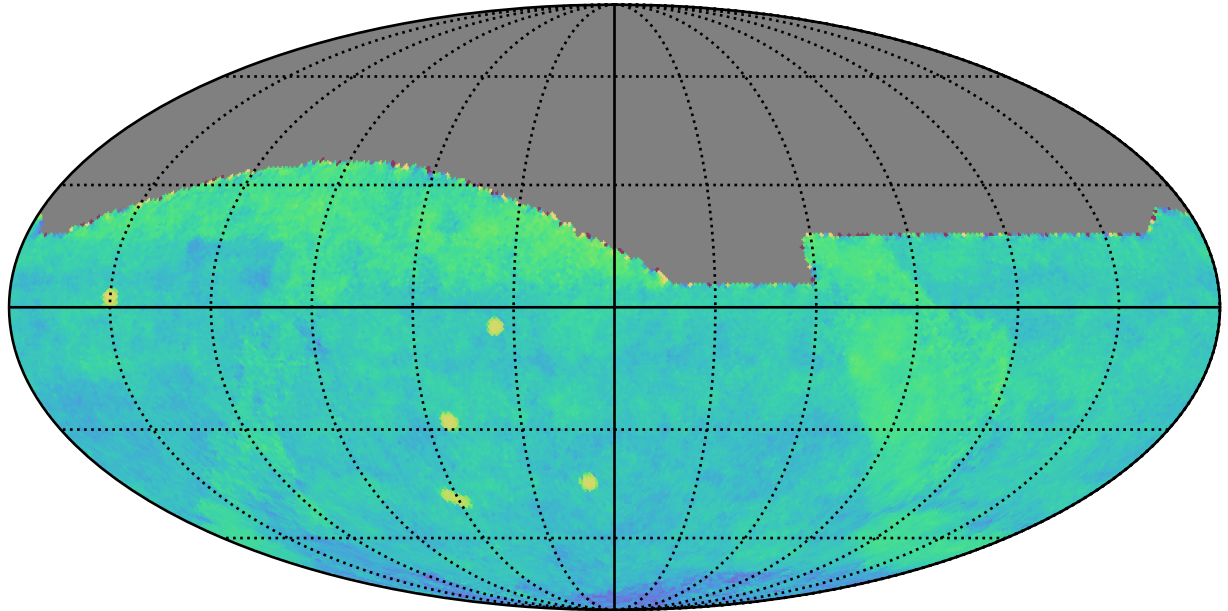
too_elab_r16_d2_gz_v3.4_10yrs gri All sky: Fraction of visits in pairs (10-60 min)
