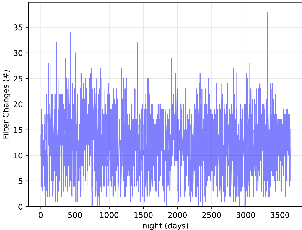
too_elab_r16_d2_gz_v3.4_10yrs Per Night: Filter Changes
