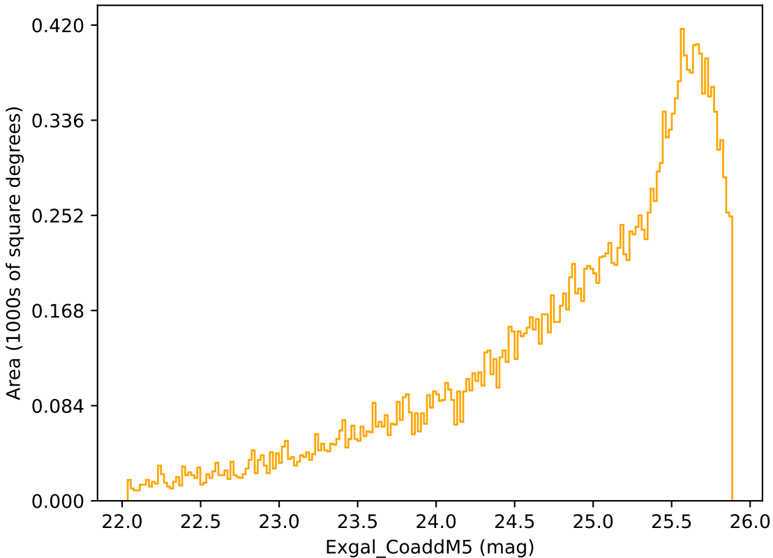
too_elab_r16_d2_gz_v3.4_10yrs Yr 3-4 r band: Exgal_CoaddM5
