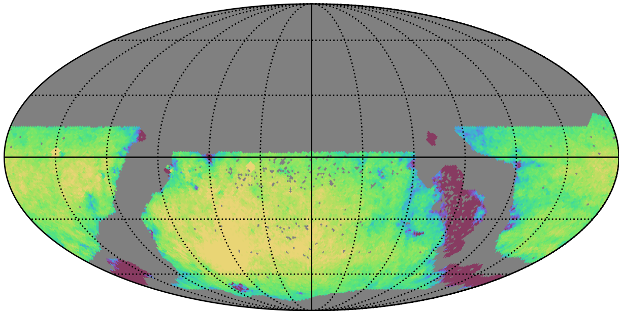
too_elab_r16_d2_gz_v3.4_10yrs WFD g band: Exgal_CoaddM5
