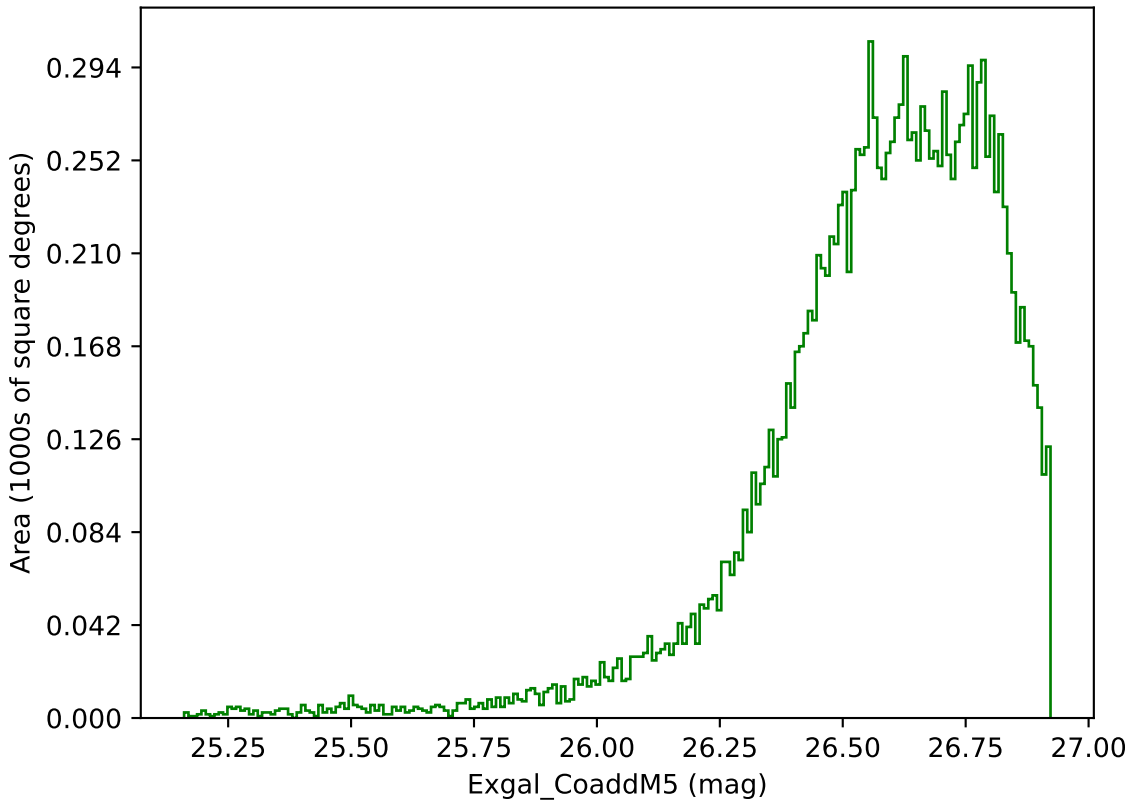
too_elab_r16_d2_gz_v3.4_10yrs WFD g band: Exgal_CoaddM5
