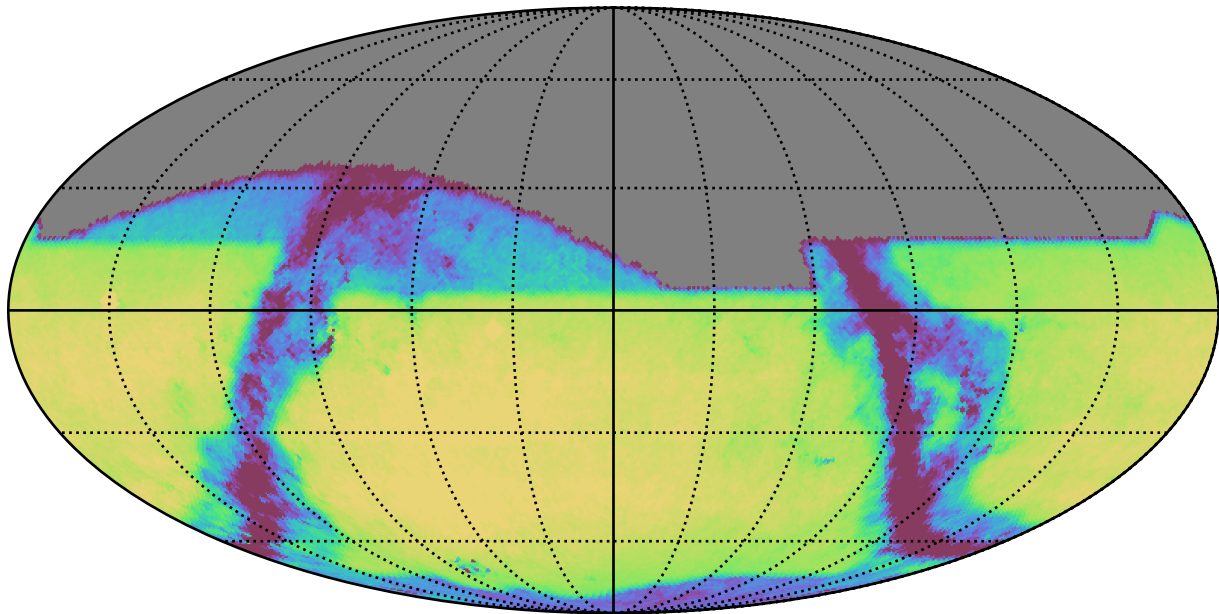
too_elab_r16_d2_gz_v3.4_10yrs All sky z band: Exgal_CoaddM5
