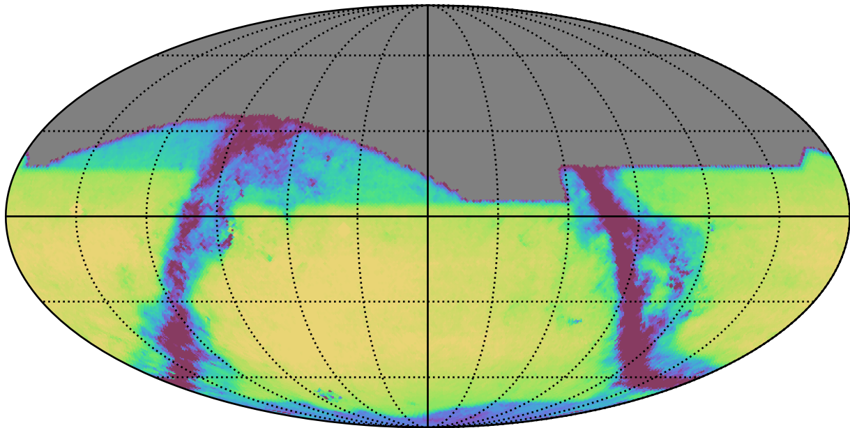
too_elab_r16_d2_gz_v3.4_10yrs All sky i band: Exgal_CoaddM5
