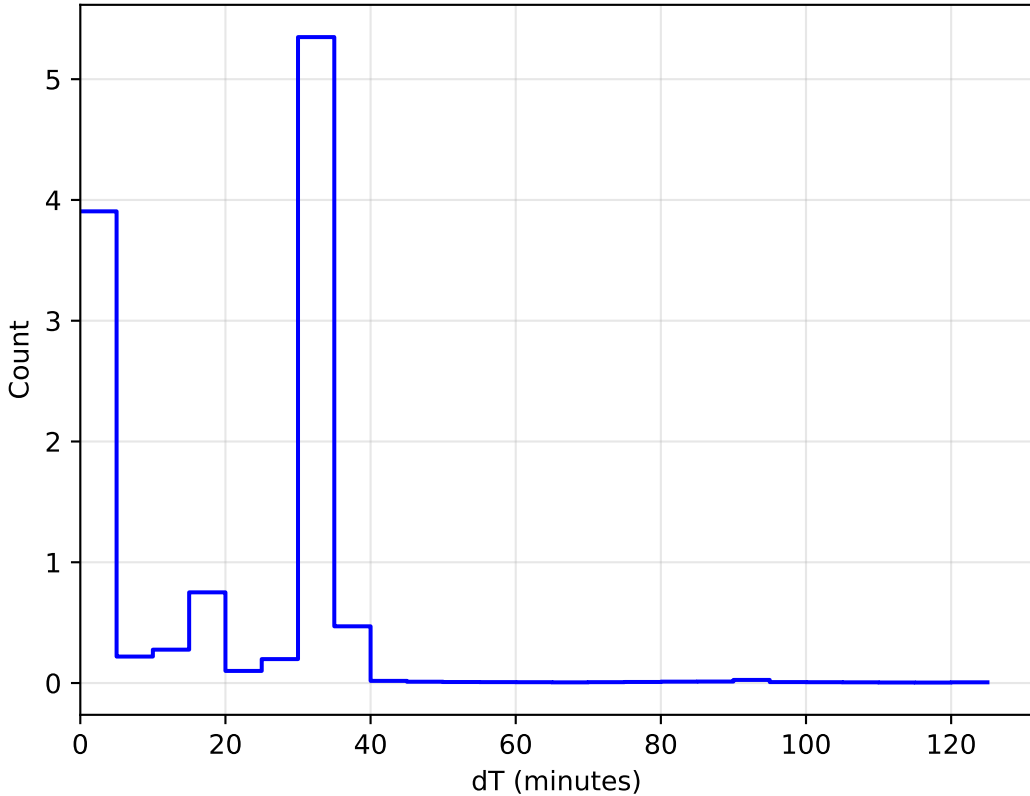
too_elab_r16_d2_gz_v3.4_10yrs WFD: DeltaT Histogram
